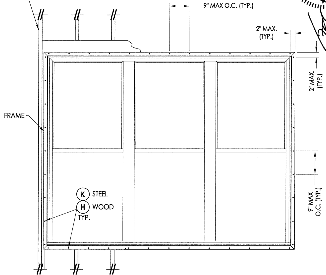
FRAME ANCHORING Stud Construction
