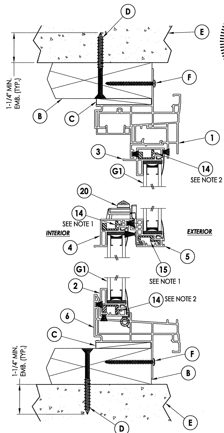
2 VERTICAL CROSS SECTION 2x Buck Construction
